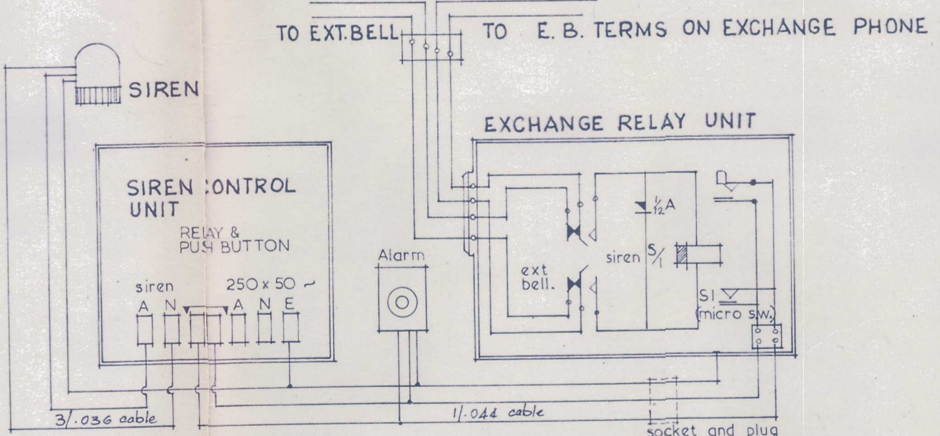
SIREN REMOTE SWITCHING BY TELEPHONE
